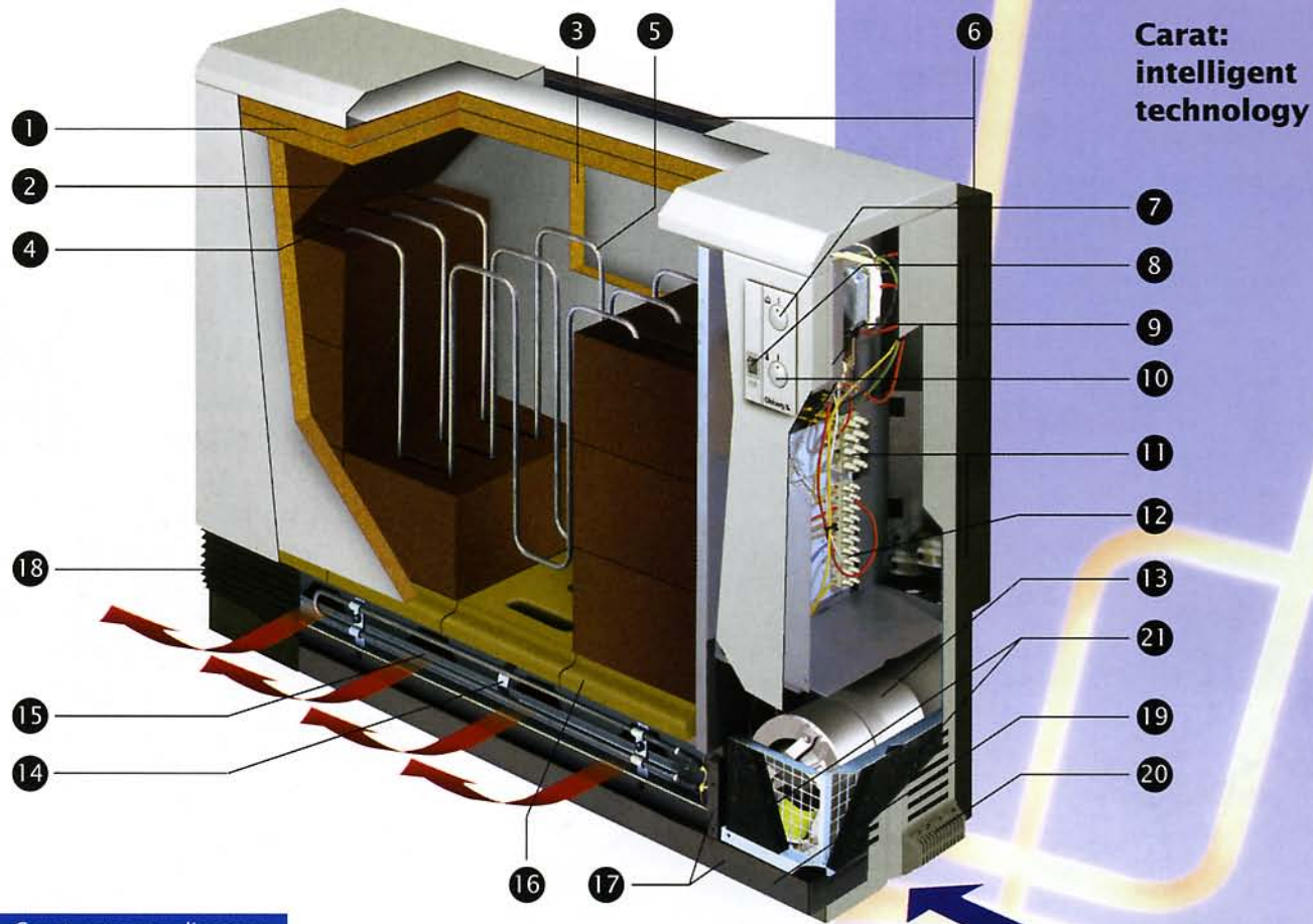
Carat cut-away diagram
