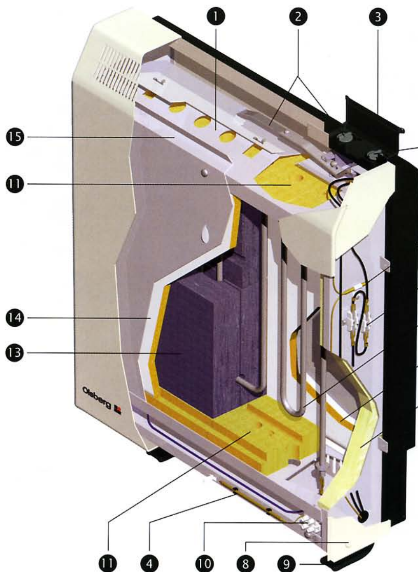
Astral cut-away diagram
